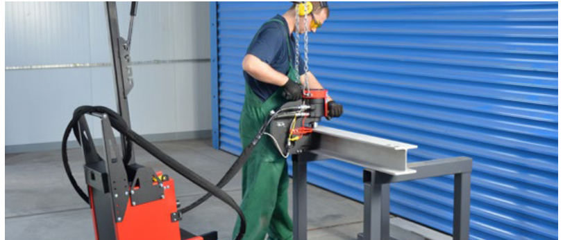
Hoist arm and 2 supports with wheels allow for easy manipulation of punch and power pack as single unit.
